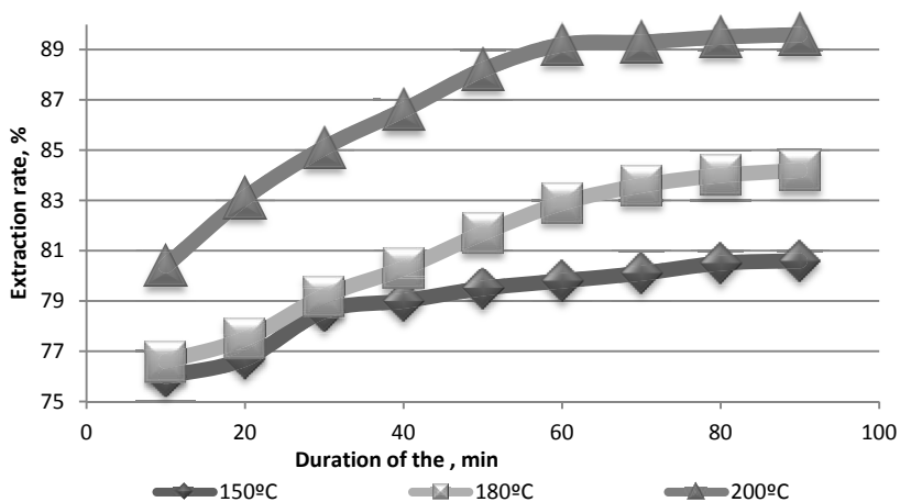
Fig. 1. Change in the extraction rate of gold in time at temperatures: 150°C; 180°C; 200°C
