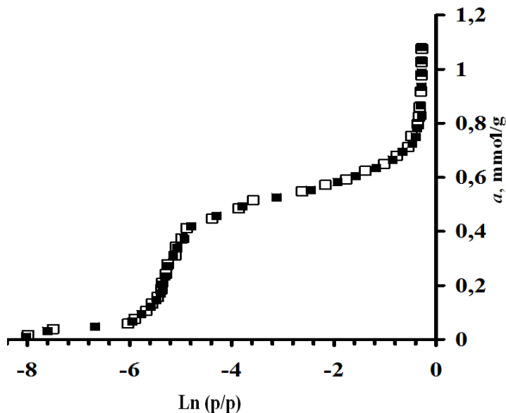
Fig. 2. Adsorption isotherm of ortho-xylene in H_{3,25}ZSM-5 zeolite at 303K □ – experimental data; ■ – points calculated by VOM
