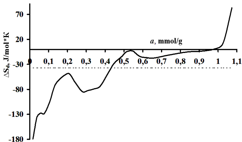
Fig. 3. The differential entropy of adsorption of ortho-xylene in H_{3,25}ZSM-5 zeolite at 303K. Entropy of liquid ortho-xylene is taken as zero. The horizontal dashed line is the middle molar integral entropy
