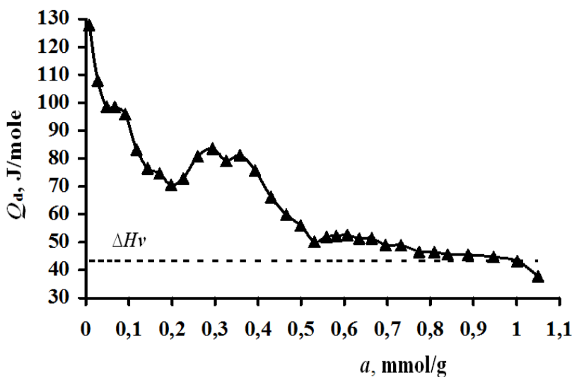
Fig. 1. The differential heat of adsorption of ortho-xylene in the H_{3.25}ZSM-5 zeolite at 303K. Dashed line is the heat of condensation of ortho-xylene at 303 K
