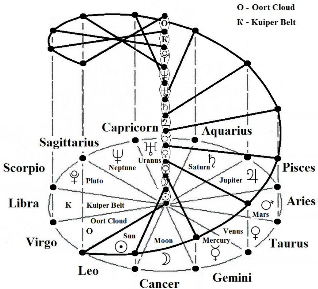
Fig. 2. 3D-spatial dependence of the effect of electromagnetic radiation in the form of the order of the qualities of the planets in the context of the axial field on the spatial characteristics, in particular, in the conventional astronomical sky concept on the division of the zodiac signs
